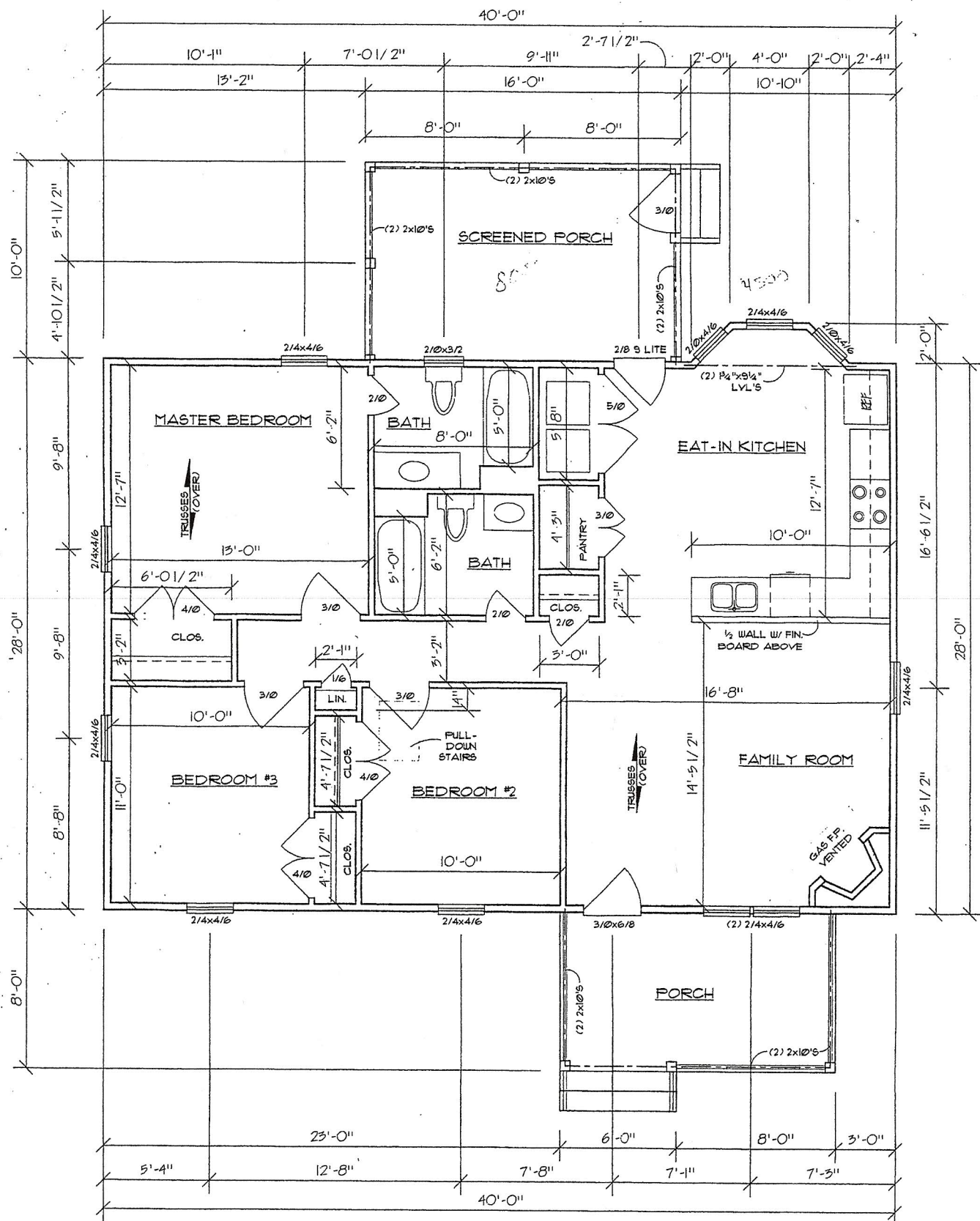
FLOOR PLAN 1132 SQ. FT. (HEATED) 112 SQ. FT. (FRONT PORCH) 160 SQ. FT. (SCREEN PORCH)
